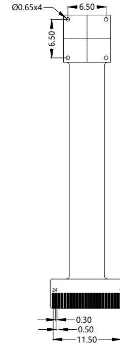
BOTTOM VIEW
